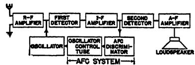
Automatic frequency control applied to a superheterodyne receiver.
